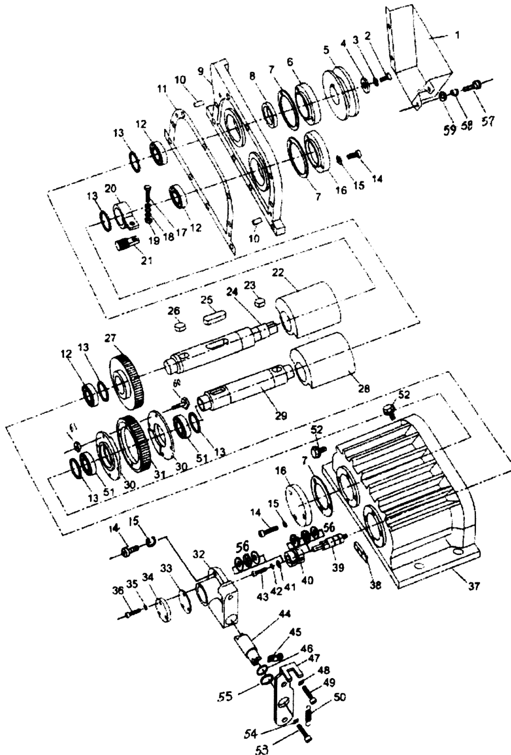
HGC125 PARTS LIST 2
